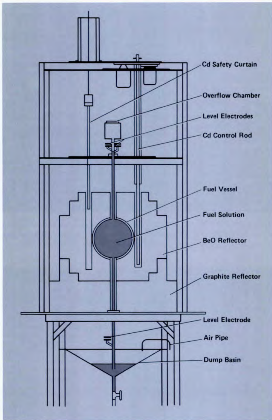
Fig. 1. Cross section of LOPO. This assembly was located inside a cubical fiberboard enclosure, 12 feet on a side, that was temperature-controlled to a fraction of a degree. Such a precaution was deemed necessary since no information existed about the temperature dependence of the reactivity.
